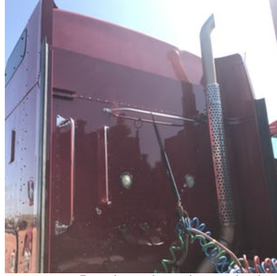
Upper reflective sheeting missing on back of cab (Requires 1' white vertical and horizontal strips in upside down L shape)
